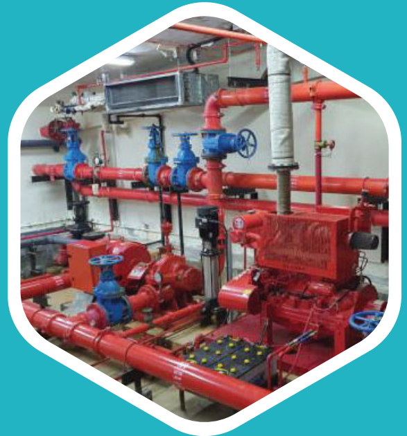
Fire Fighting Installation
