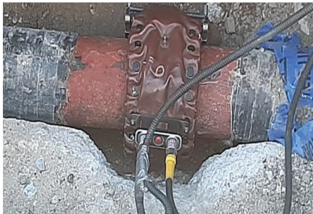
LRUT Inspection of Underground Piping
